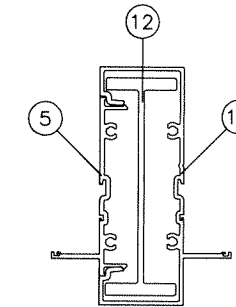
MULLION 'M2A'
