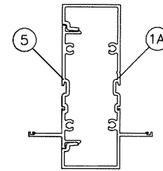
MULLION 'M1A'
