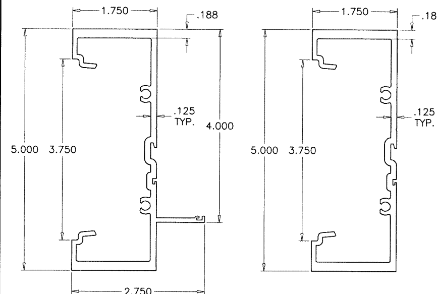
③ FRAME JAMB/MULLION
