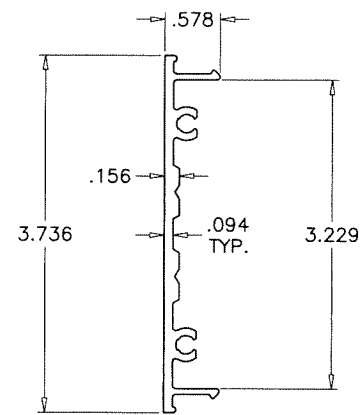
⑥ SHEAR CLIP
