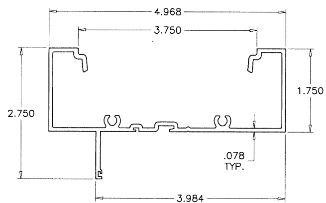
①A FRAME HEAD/SILL/JAMB/MULLION
